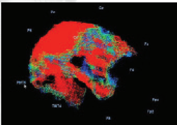
sLORETA 3-D Head Display
