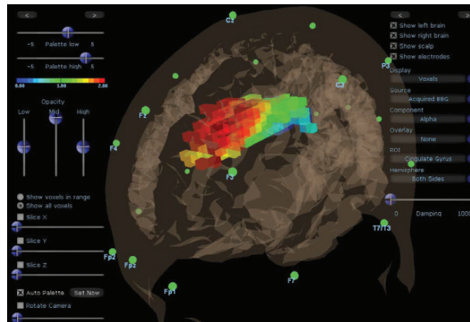
Above: A live reconstruction and imaging using sLORETA. It depicts training within the Cingulate Gyrus.
